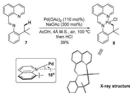
Scheme 3. Stoichiometric formation and isolation of palladacycle 8 .
